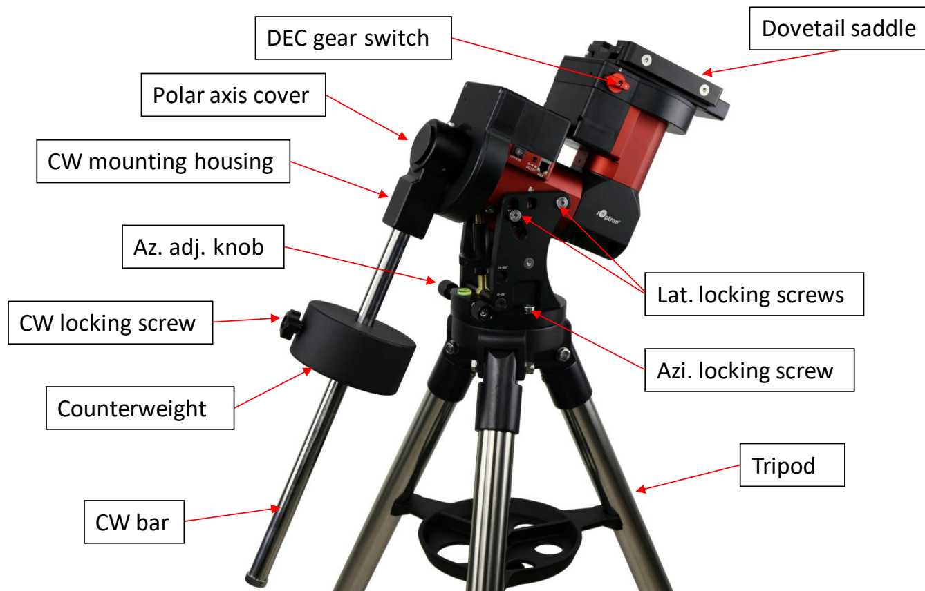
Figure 1.CEM40 mount assembly
